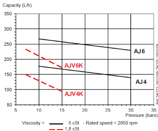
Pump capacity
