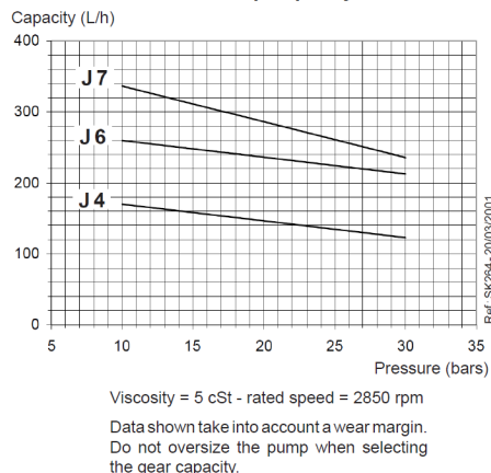
Pump capacity
