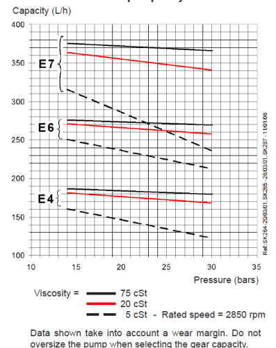
Pump capacity
