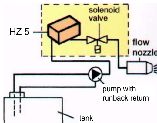
Installation Example for Pressure Operation
