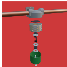
Exploded Diagram
